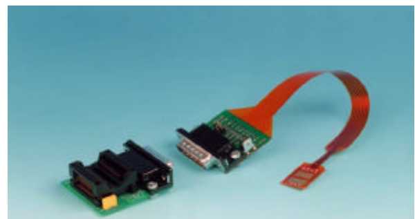
IN-GSM with IN-SO28 IN-GSM Interface adapter with SIM/GSM format contacts.
