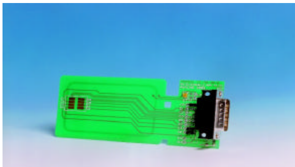
IN-CLA7816USB Interface adapter containing ISO7816 format contacts, USB interface and contactless antenna.
